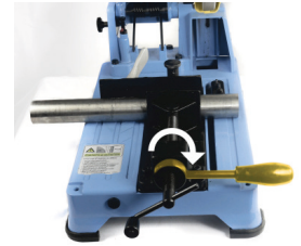
5. Turn the lever to the right and start the sawing process: next steps: 3 - 4 - 5.
