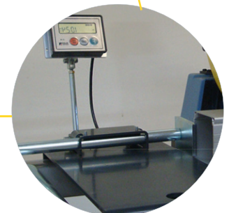
Variant B: DIGITAL, with digital measuring range display Art. 609960 B
