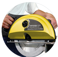
Saws sheet metal up to 10 mm and sandwich panels and profiles with a cutting depth of up to 67 mm
