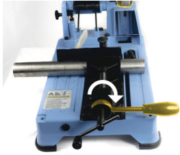
1. Starting position: The quick release lever is on the right.
